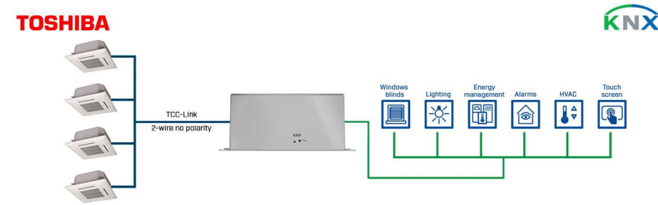
Use Case Integration of Toshiba VRF systems into a KNX installation.
