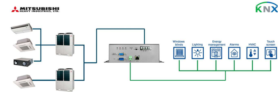
Use Case Integration of Mitsubishi Heavy Industries Air Conditioner Units through Superlink connection into a KNX installation.
